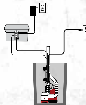
Regular Installation
