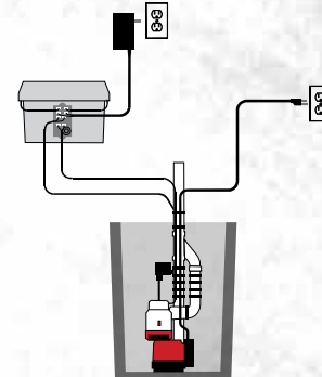
Alternate Installation
